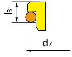
TS551D G6 (DIN24960)
